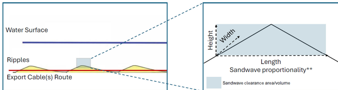
*Figures show the sandwave profile viewed parallel to the shoreline. ** Proportionality represents the % of route requiring sandwave clearance
