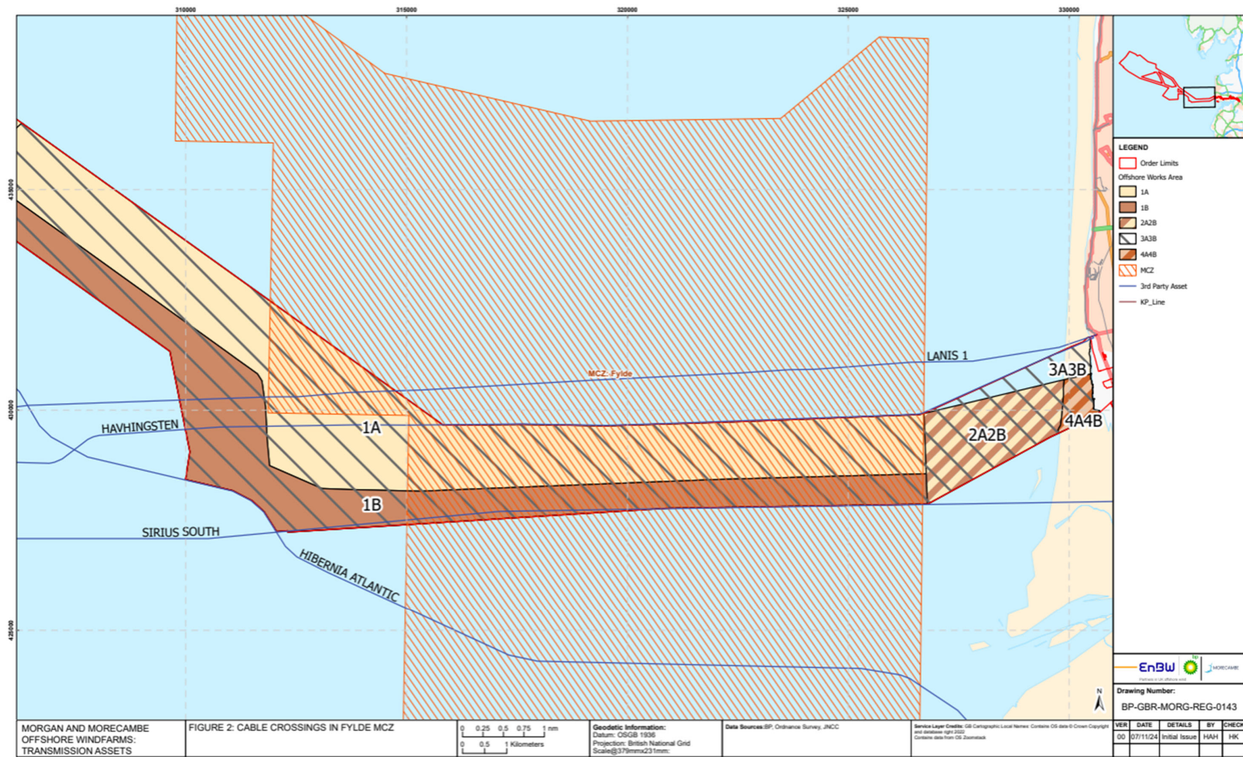
Figure 2: Cable crossings in Fylde MCZ
