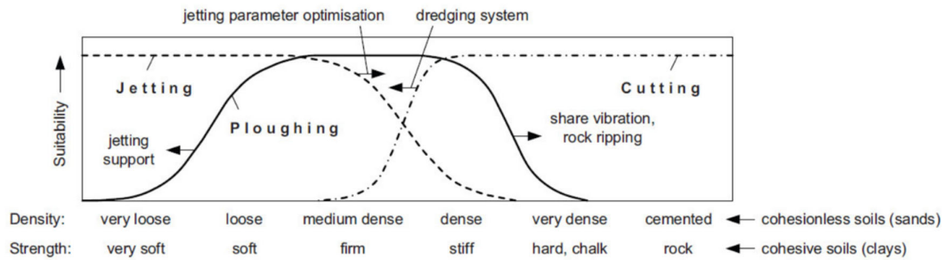
Figure 5: Burial Technique Suitability (DVNGL 2016)
